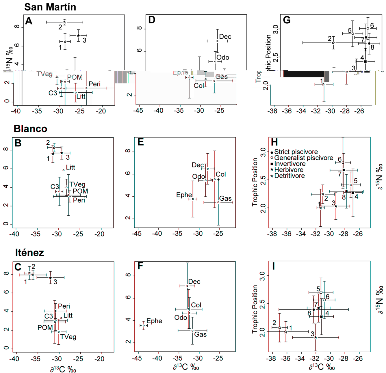
Figure 2. Isotopic signature of sources, invertebrates and fish in three rivers of the Iténez basin (Amazon, Bolivia). Biplots display mean values ( \pm sd in error bars) of \delta^{13}\text{C} and \delta^{15}\text{N} values for sources (A,B,C) POM = Particulate organic matter, Litt = Leaf litter, Peri = Periphyton; C3 = C3 aquatic macrophytes and TVeg = Terrestrial Vegetation; and invertebrates groups (D,E,F): Ephe = Ephemeroptera, Odo = Odonata, Dec = Decapoda, Col = Coleoptera and Gas = Gasteropoda. (G,H,I) represented mean values ( \pm sd in error bars) of \delta^{13}\text{C} and Trophic Position (derived from \delta^{15}\text{N} ) of fish species: detritivore (1 = Curimatella cf. albuna , 2 = Psectrogaster sp.), herbivore (3 = Schizodon fasciatus ), insectivore (4 = Triporthus angulatus ) and piscivore (5 = Pseudoplatystoma sp., 6 = Pygocentrus nattereri , 7 = Hoplias malabaricus and 8 = Acestrorhynchus sp.). In biplots (A,B,C), C4 aquatic macrophytes ( \delta^{13}\text{C} : -12.3 to -13.2\text{‰} ; \delta^{15}\text{N} : 2 to 2.2\text{‰} ) were not plotted and \delta^{13}\text{C} and \delta^{15}\text{N} values of detritivore (1, 2) and herbivore (3) fish species were reported. doi:10.1371/journal.pone.0065054.g002
